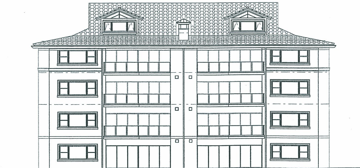
REAR ELEVATION
