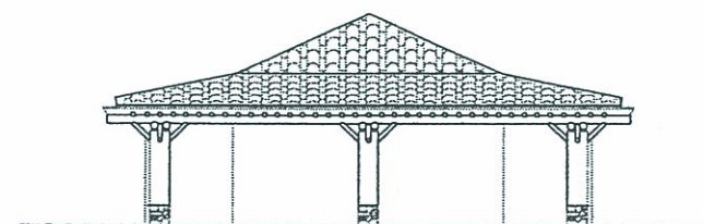
REAR ELEVATION
